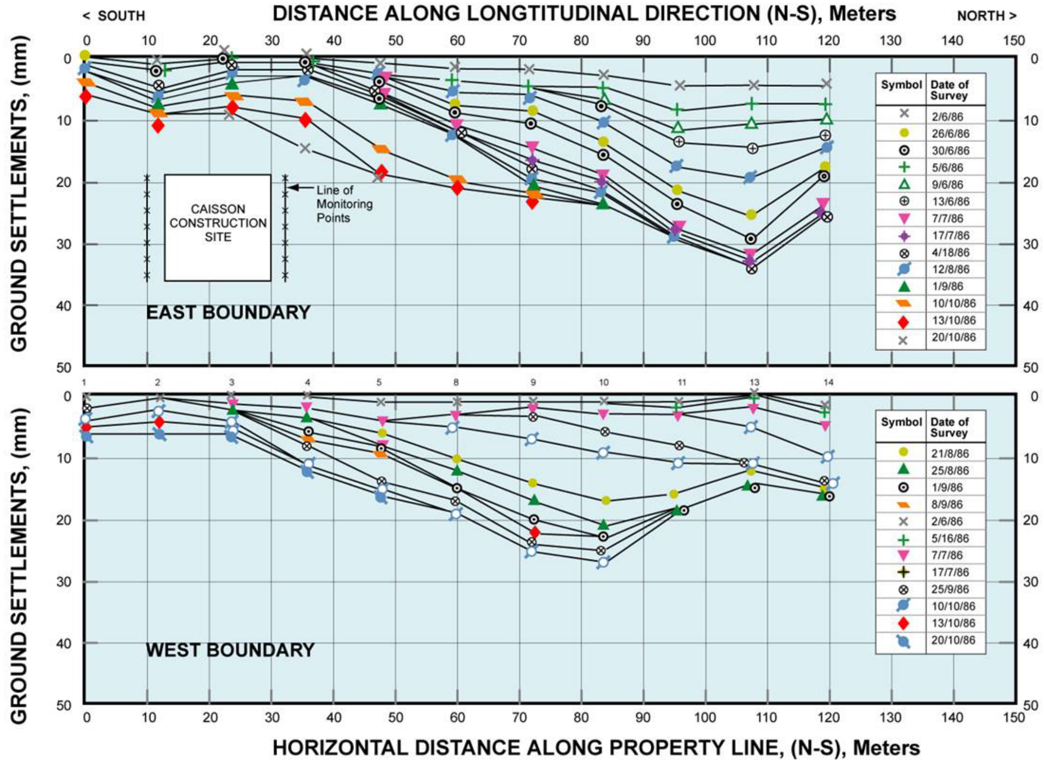
GROUND SETTLEMENT DURING INSTALLATION OF BORED PILES PHASE II FOUNDATIONS
