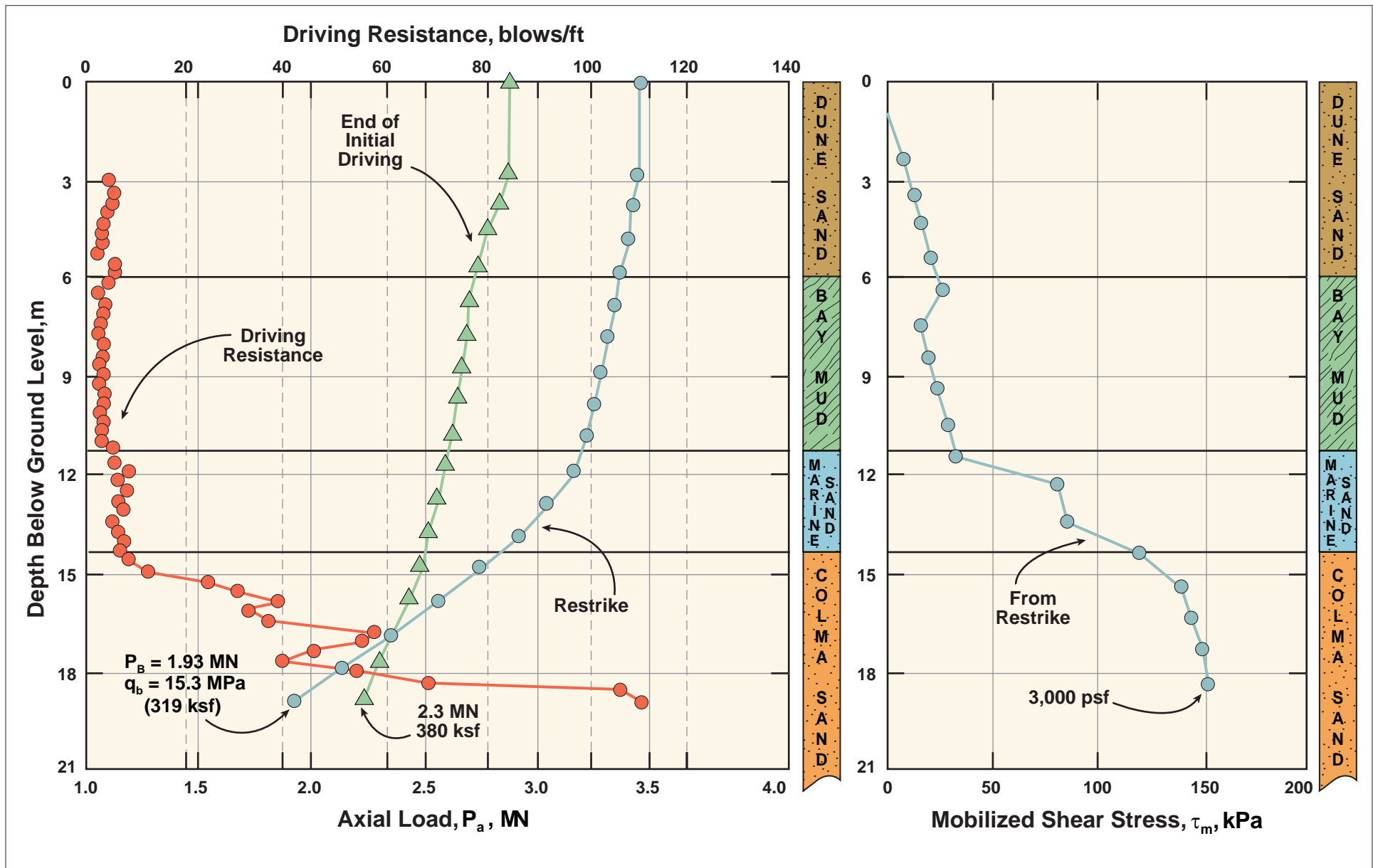
Plate Q-04: Axial Load Distribution, Mobilized Skin Friction and End-Bearing Resistance from PDA Tests: Site No. 1, Indicator Pile No. IP-13
