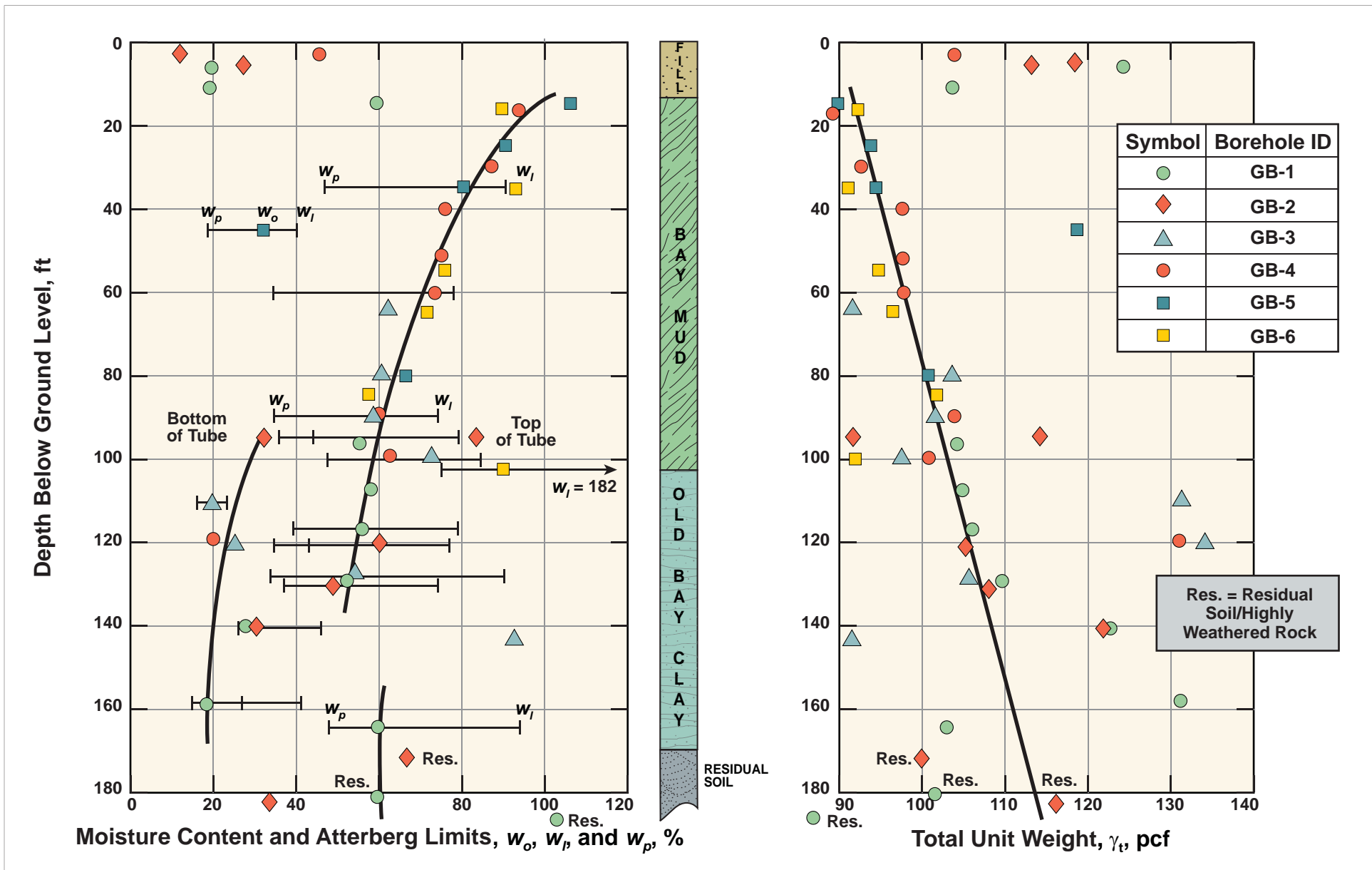
Plate K-05: Moisture and Density Profiles
