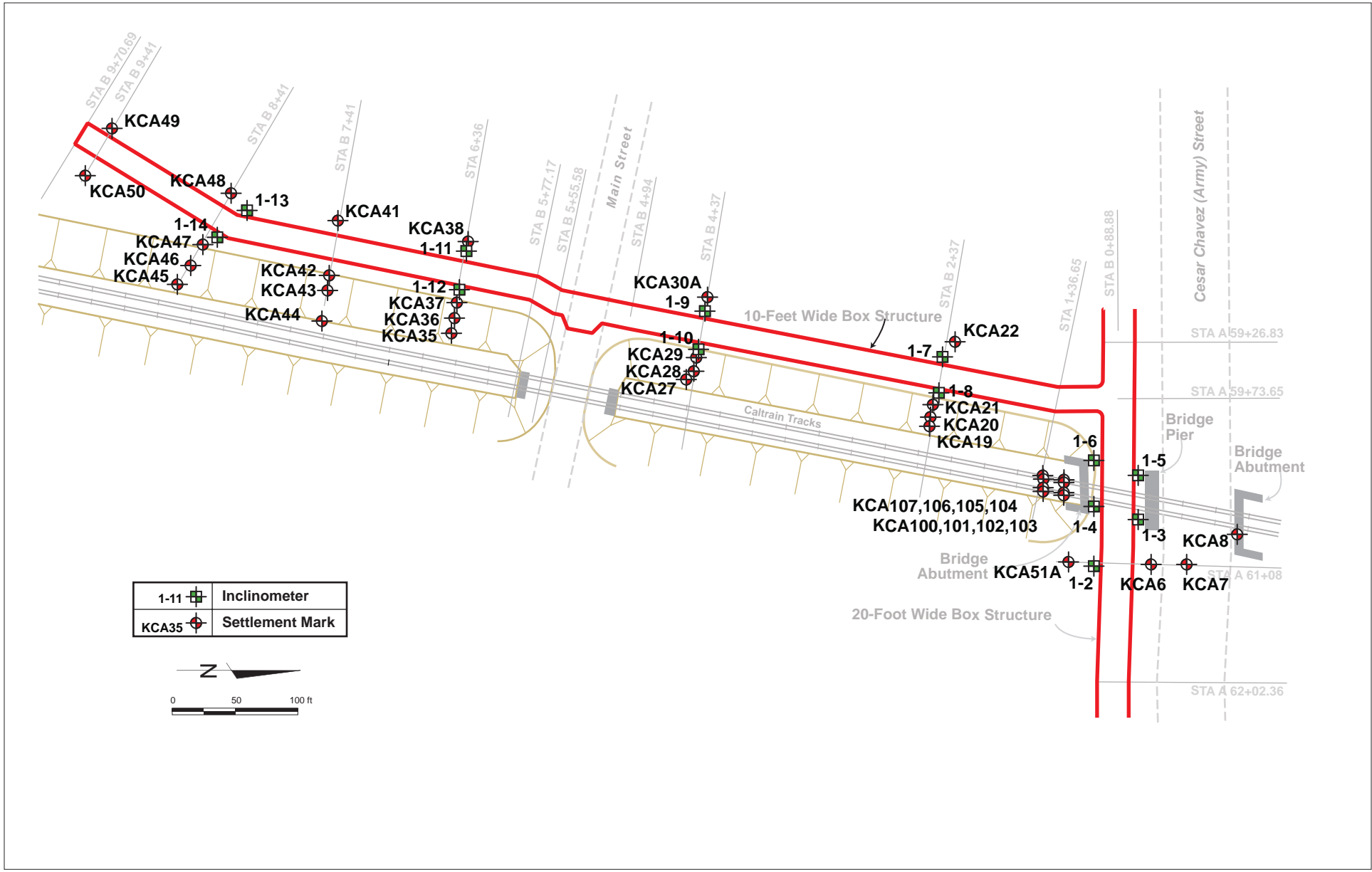
Plate D-05: Instrumental Plan
