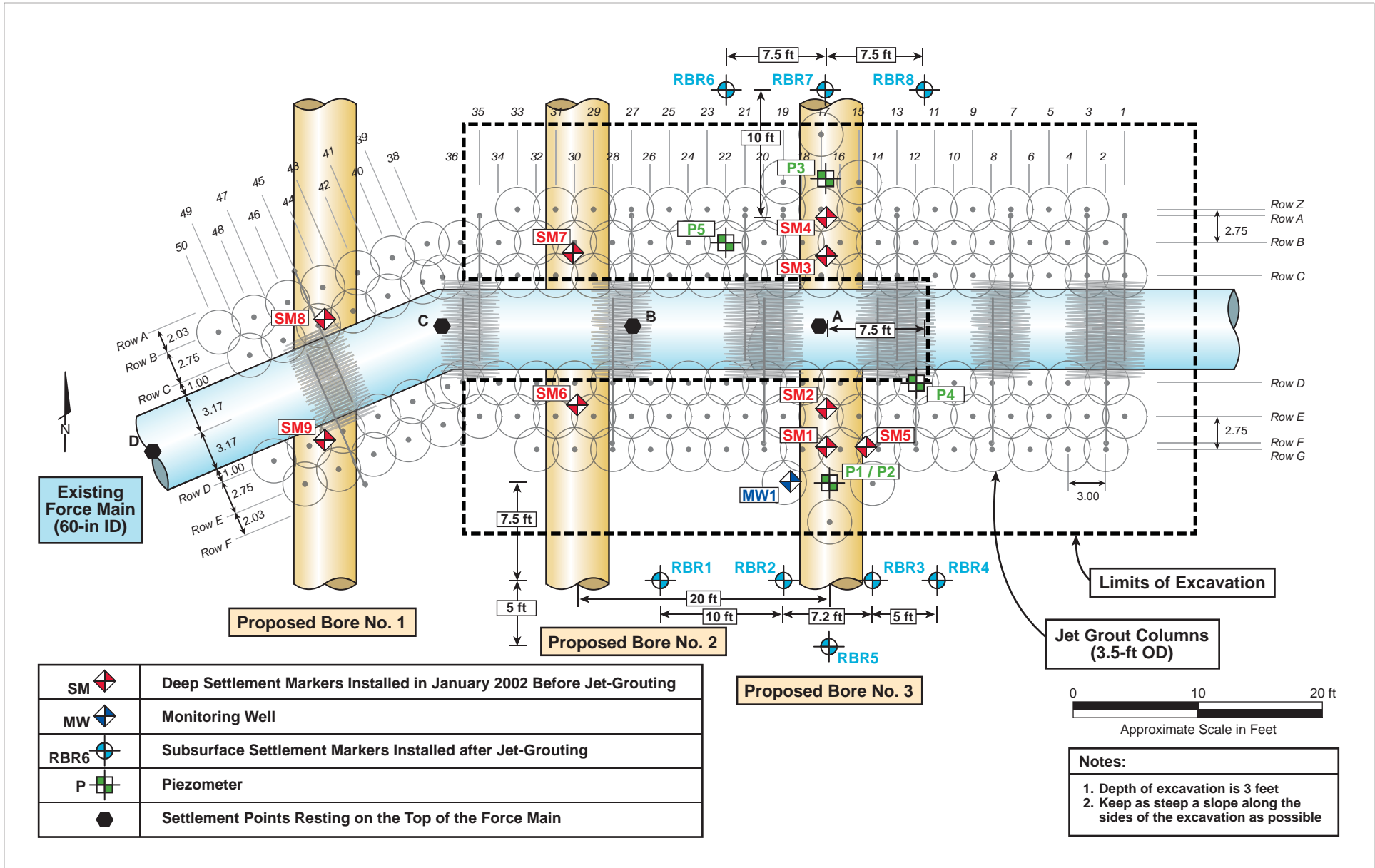
Plate C-15: Excavation Plan
