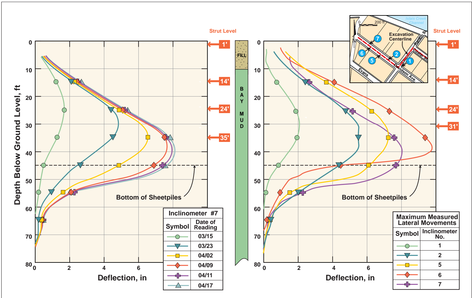
FIG_F-01: Figure A: Typical Measured Lateral Movements for Deepening Excavation on Davidson Avenue-Inclinometer No. 7 Figure B: Maximum Measured Lateral Movements in All Inclinometers Except Nos. 3 and 4
