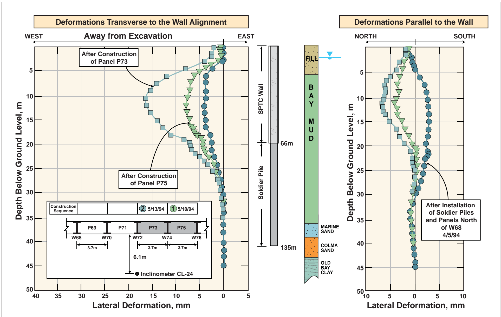
FIG_201C: Lateral Deformations During SPTC Wall Construction
